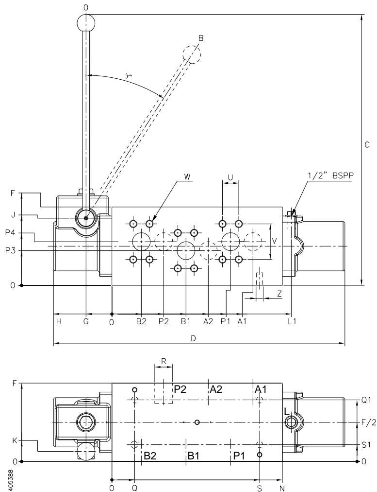
Figure 2 13STF Dimensions
