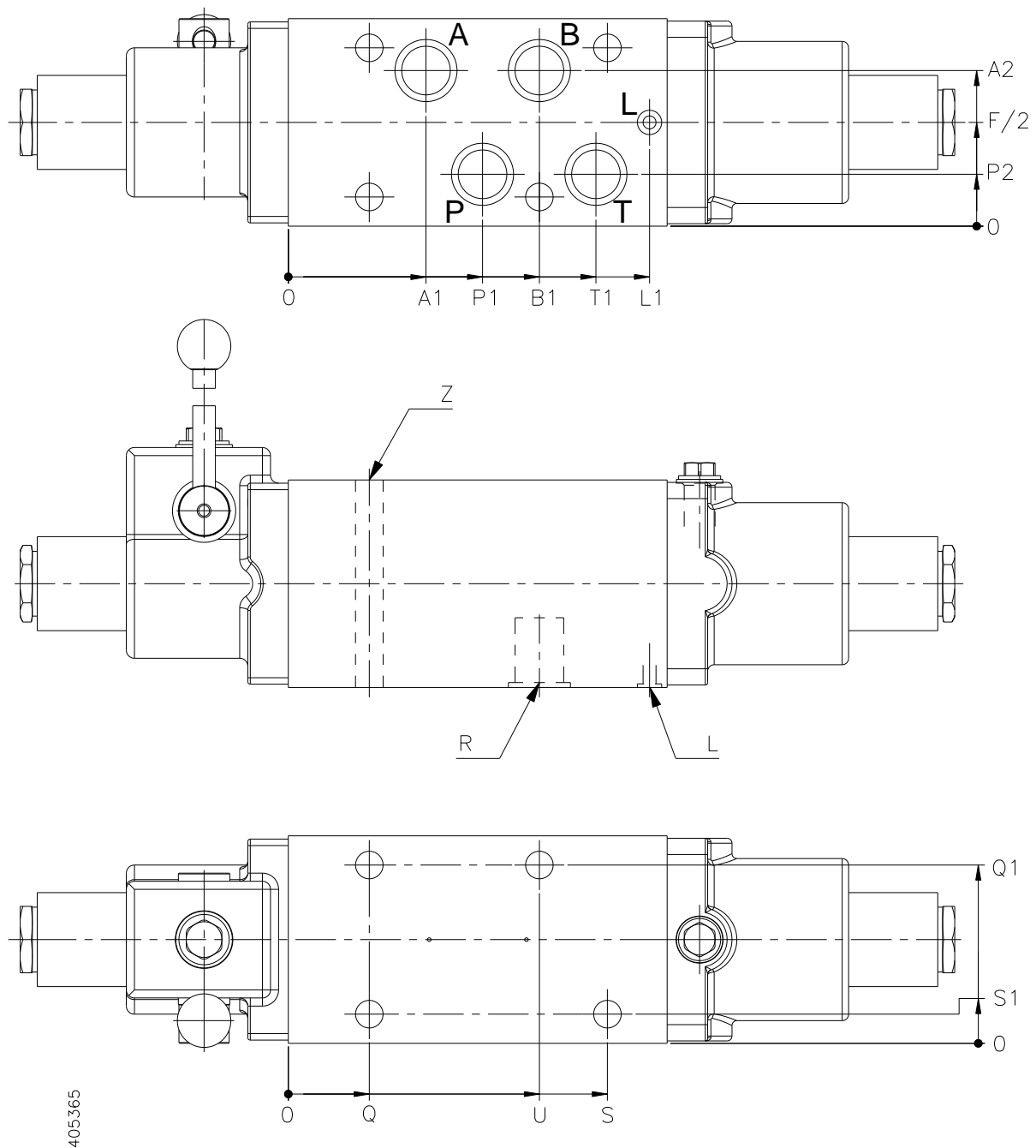
Figure 4 20STB Dimensions
