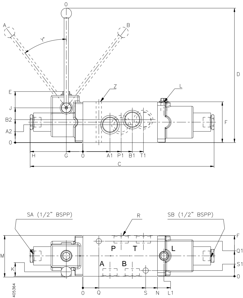
Figure 2 20ST Dimensions
