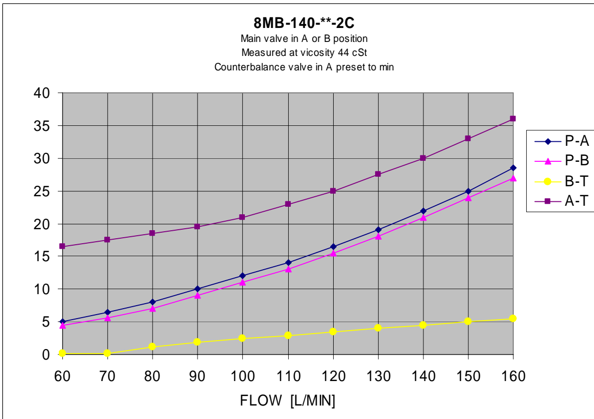
Figure 6 8MB-140-**-2C-MA pressure drop
