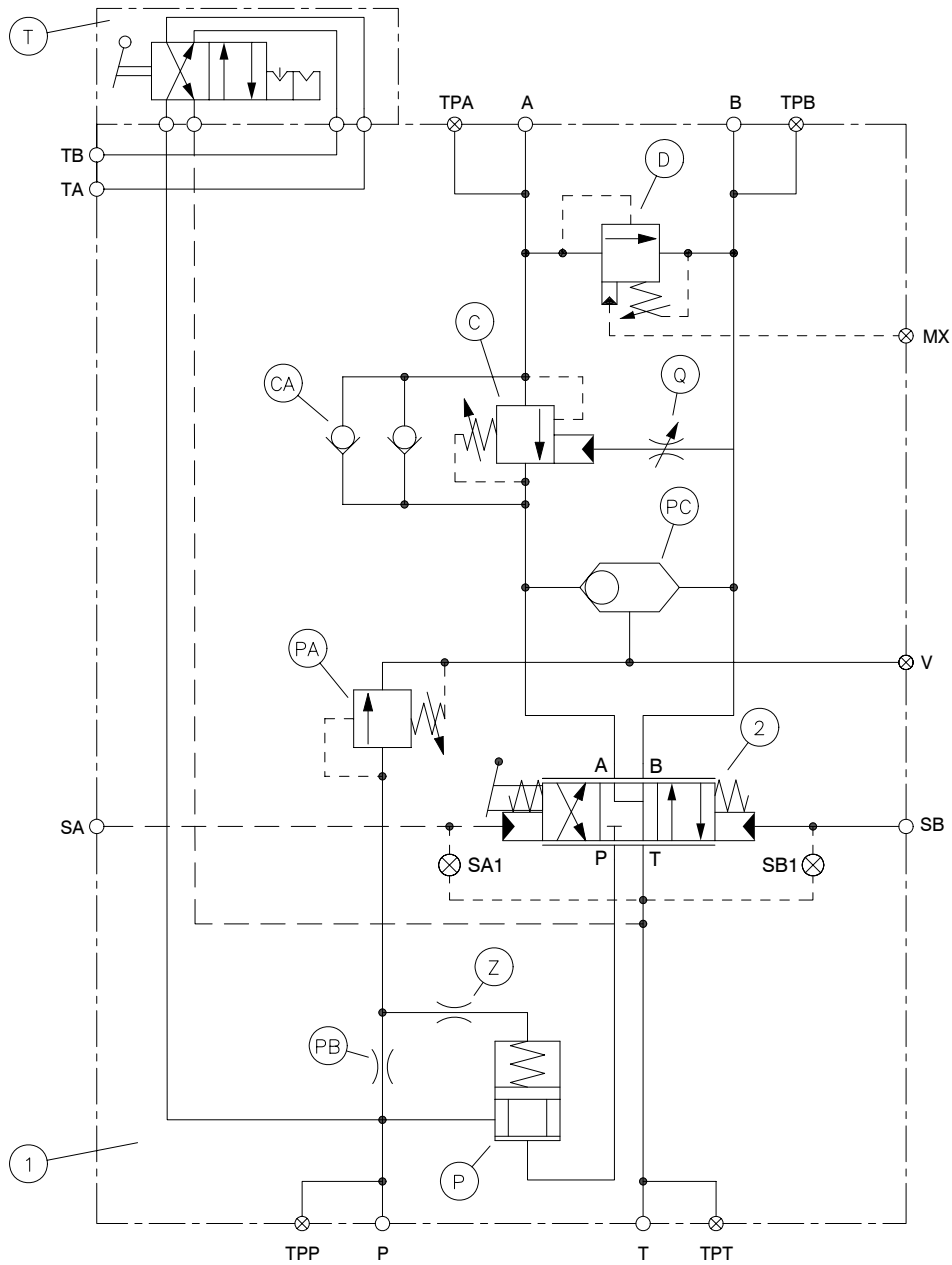
Figure 3 Hydraulic Schematic 8MB-***-37-2C-MA-T
