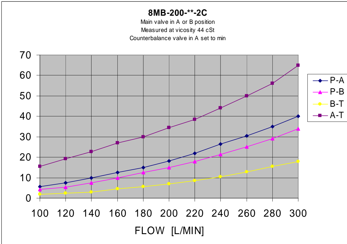
Figure 5 8MB-200-**-2C-MA pressure drop
