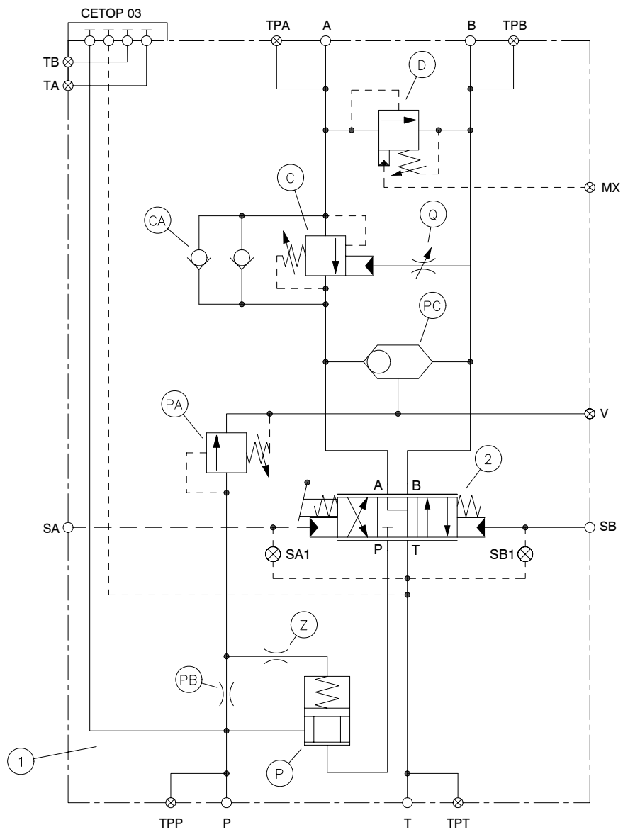
Figure 2 Hydraulic Schematic 8MB-200-37-2C-MA
