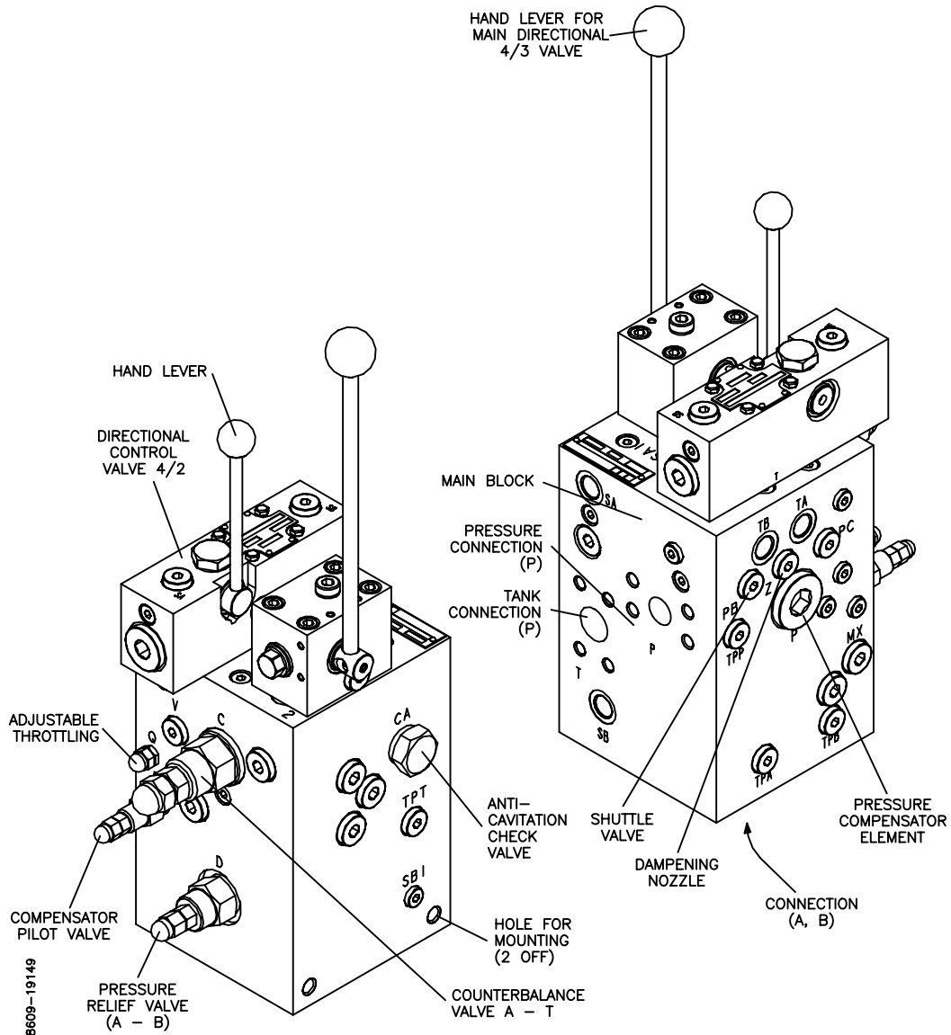
Figure 1 General Arrangement 8MB-***-**-2C-MA-T
